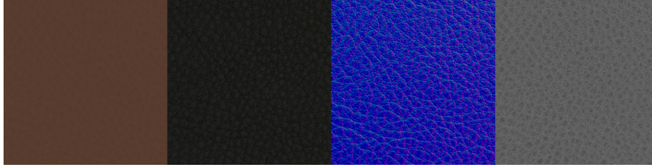
Figure 3: The standard SVBRDF (isotropic Ward) parameter textures of a measured leather material (from left to right): diffuse , specular , normal , roughness .
