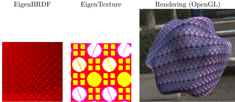
Figure 8: The first three angular and spatial components of a factorized BTF encoded in a color mapped RGB image. The right image shows a rendering of the material.
